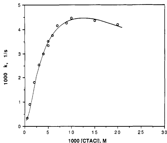
Figure 2. Pseudo-first-order rate constants ( k_p , s^{-1} ) for the cleavage of 1 \times 10^{-5} M PNPDP by 1 \times 10^{-4} M 4 as a function of [CTACl] at pH 8; see text for other conditions. Each reaction was followed spectrophotometrically, monitoring the release of p -nitrophenoxide ion at 400 nm.
