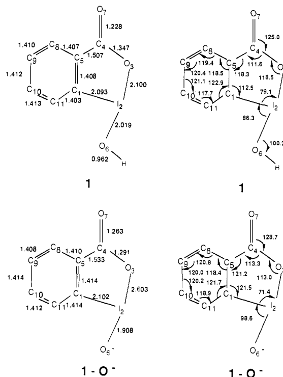
Figure 3. Calculated bond lengths and angles for the non-hydrogen atoms in the conjugate acid/base pair 1/1-O - . The calculations are described in the text. Full sets of Cartesian coordinates are available in the supplementary material.
