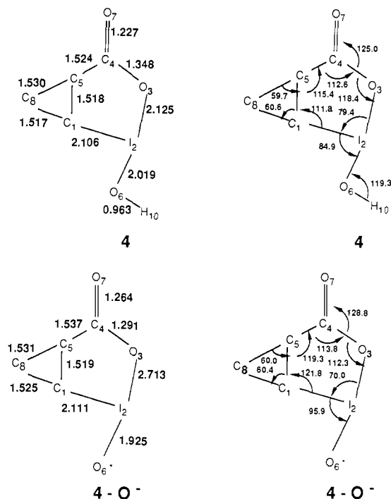
Figure 4. Calculated bond lengths and angles for the non-hydrogen atoms in the conjugate acid/base pair 4/4-O - . The calculations are described in the text. Full sets of Cartesian coordinates are available in the supplementary material.
