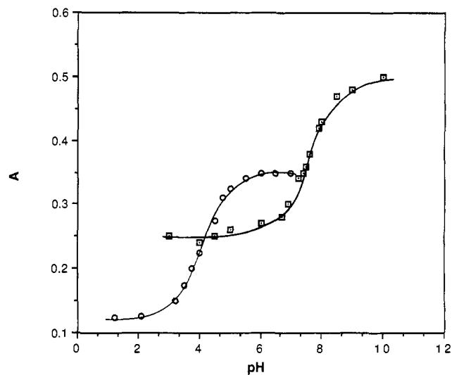
Figure 1. Spectrophotometric titrations of iodo acid 5 (O) and 1-hydroxyiodoxolone 4 (□); absorbance versus pH. The pK_a 's were 4.10 and 7.55, respectively, as determined from the linear plots of \log(A - A_{\min})/(A_{\max} - A) versus pH; thus pK_a = \text{pH} when the logarithmic quantity = 0.
